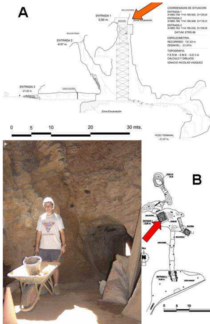
Sima de las Palomas: A elevation, B plan, Arrow points to excavation area; left, mine tunnel entrance; right, main shaft
